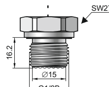
CG1/2B type G1/2" with flush diaphragm
