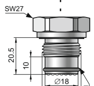
CG1/2 type G1/2" with flush diaphragm
